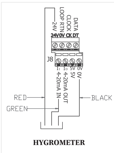
Hygrometer connection to BAS HL controller PCB.
