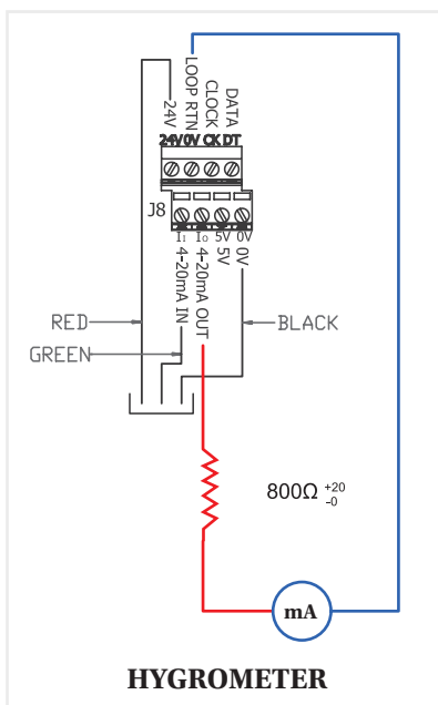
An 800Ω (+20 Ω / -0 Ω) resistor will be required in series in the loop circuit.
