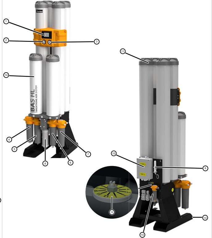
Representation of Models BAS HL075 to BAS HL085
