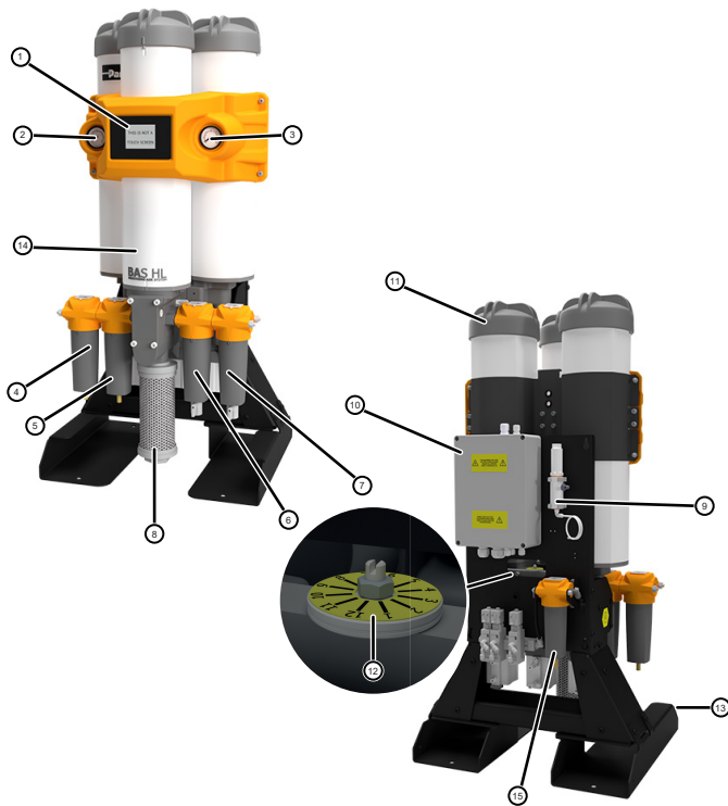
Representation of Models BAS HL050 to BAS HL070
