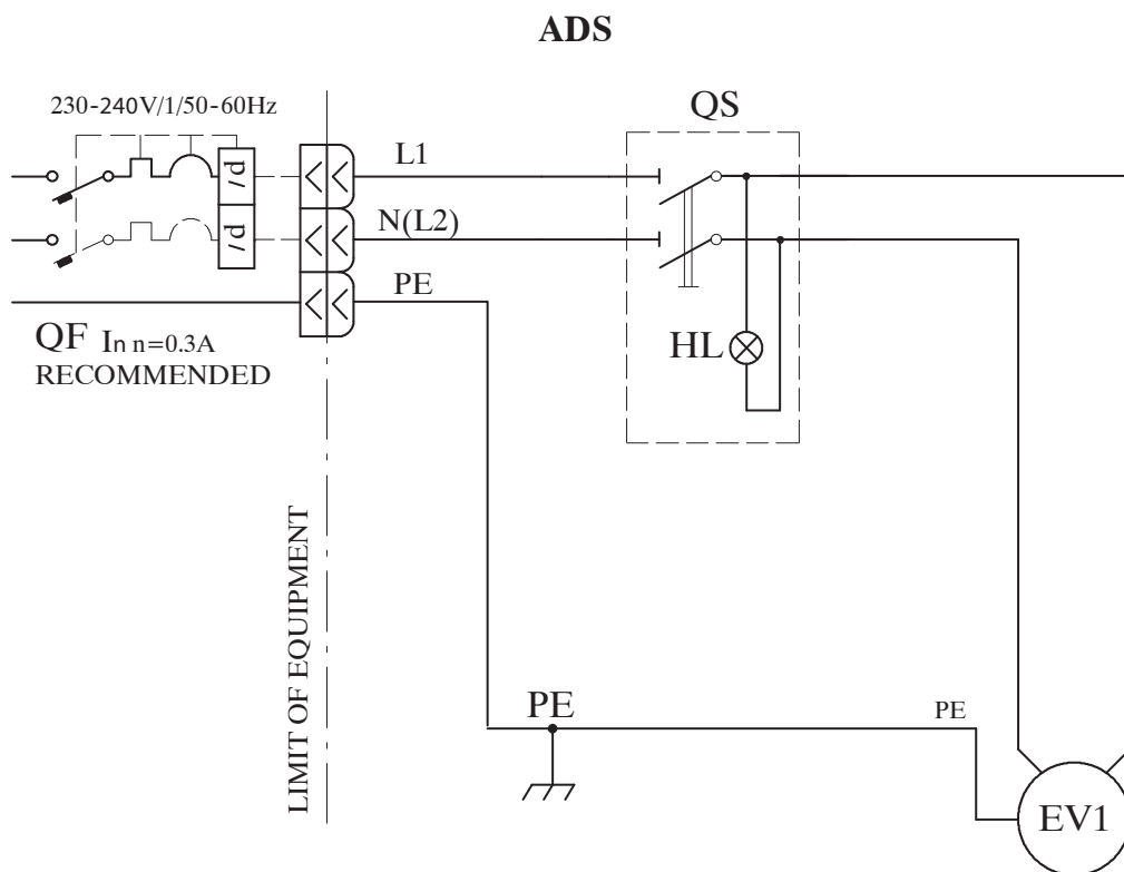
Fig. 6 – Electrical diagram
